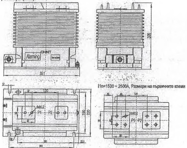
LZZBJ77-20/220b/2 NH
