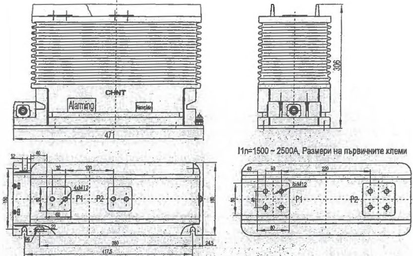
LZZBJ77-20/180b/4 NH
